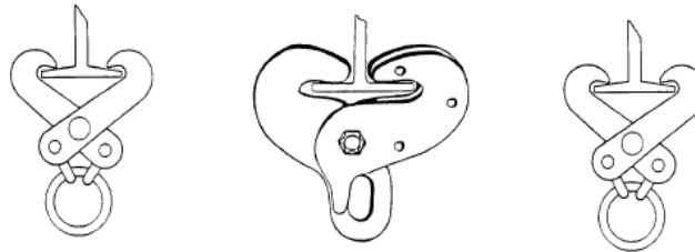
Figure 5.1 – Adjustable Type Beam Clamps
